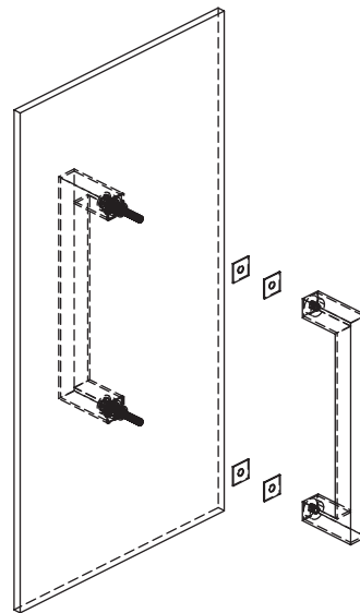
ISO EXPLODED VIEW-2
